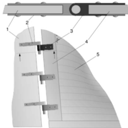
Figure 3 A pintle and gudgeon sternpost rudder. The “pintles” are the vertical pins attached to the rudder and the “gudgeons” are the iron loops attached to the sternpost of the hull. The labeled parts are: (1) the rudder, (2) a pintle, (3) a gudgeon, (4) the sternpost, and (5) the hull of the ship.
