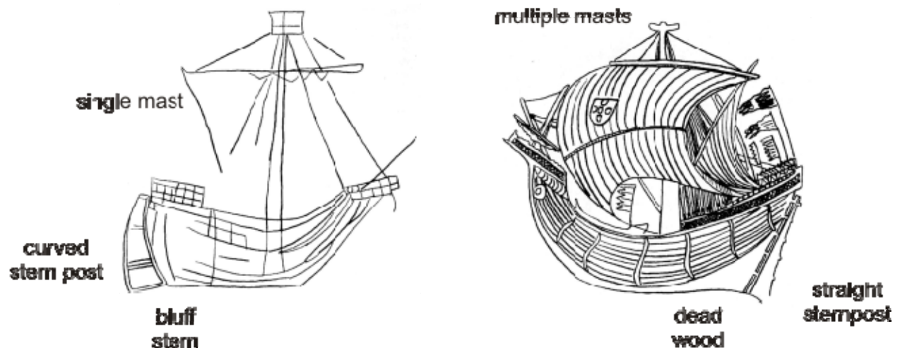
Figure 4 illustrates development of ship design after the introduction of the sternpost rudder to the Mediterranean. The left panel shows a tracing of a drawing of a medieval ship from the bell tower of the Cathedral of Palma de Mallorca that probably dates to the early 13 th century. The curved sternpost, bluff stern, and single mast were characteristic of contemporary ships with quarter rudders. Note the very broad rudder
